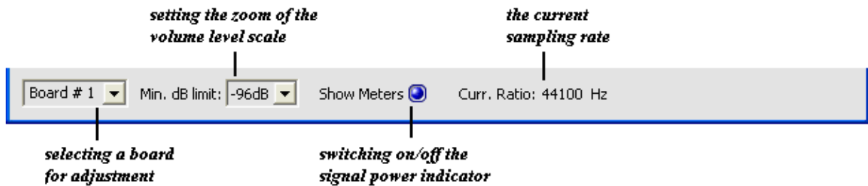
Figure 19. The Sound Configure general settings.
