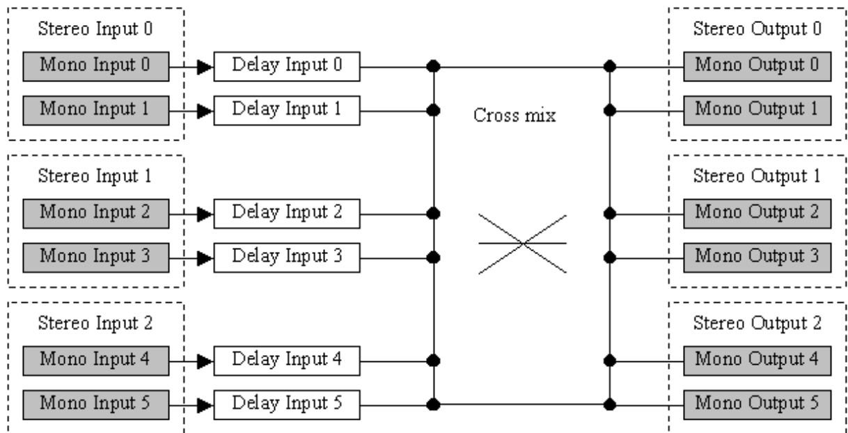
Figure 1. Sound mixing diagram.
