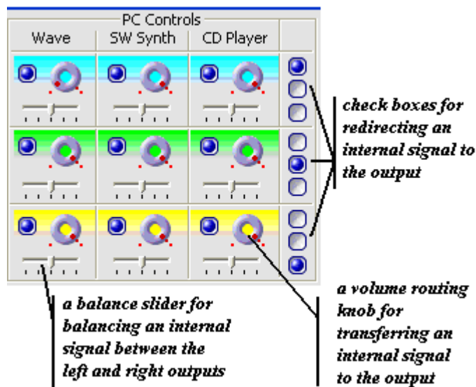
Figure 16. Mixing the internal input signals.
