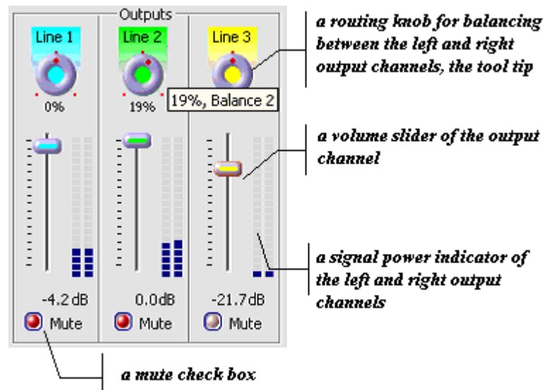
Figure 18. The controls of the output signals.
