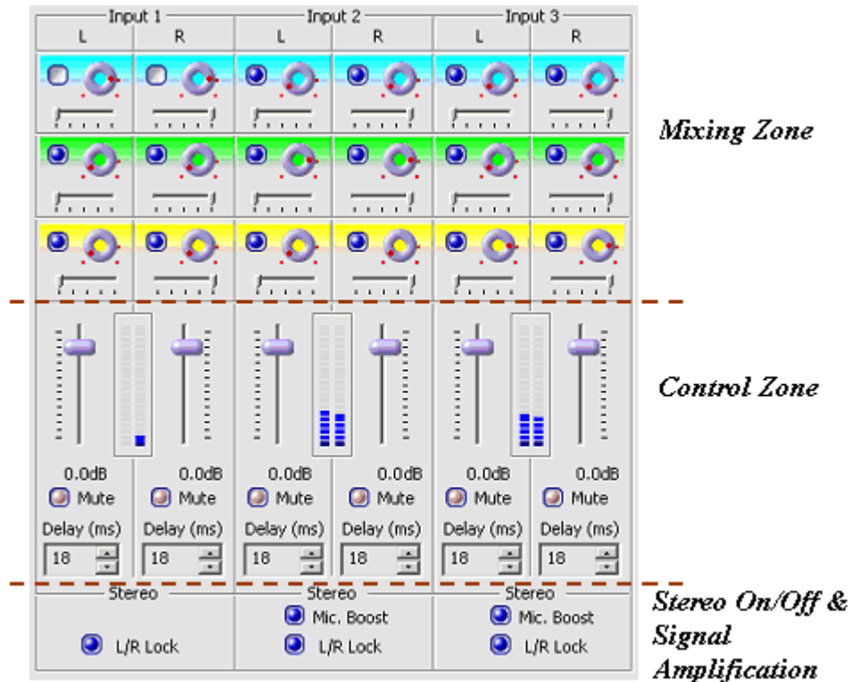
Figure 4. Control zones of the input signals.
